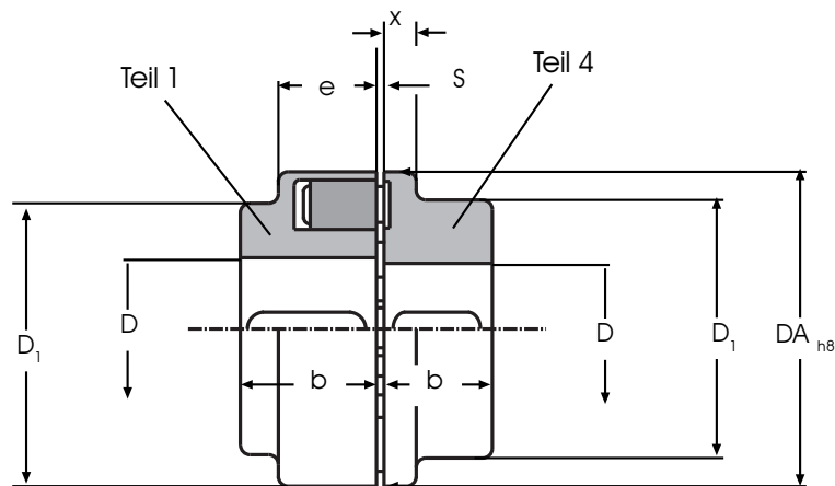
Bauart A
